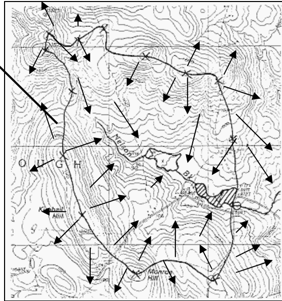
Figure 7. Delineated watershed with arrows pointing in the direction of runoff flow and X'ed hilltops and high points.
